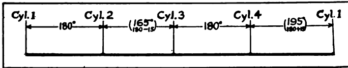
Intervals Separating Four Explosions, Aries Motor.
